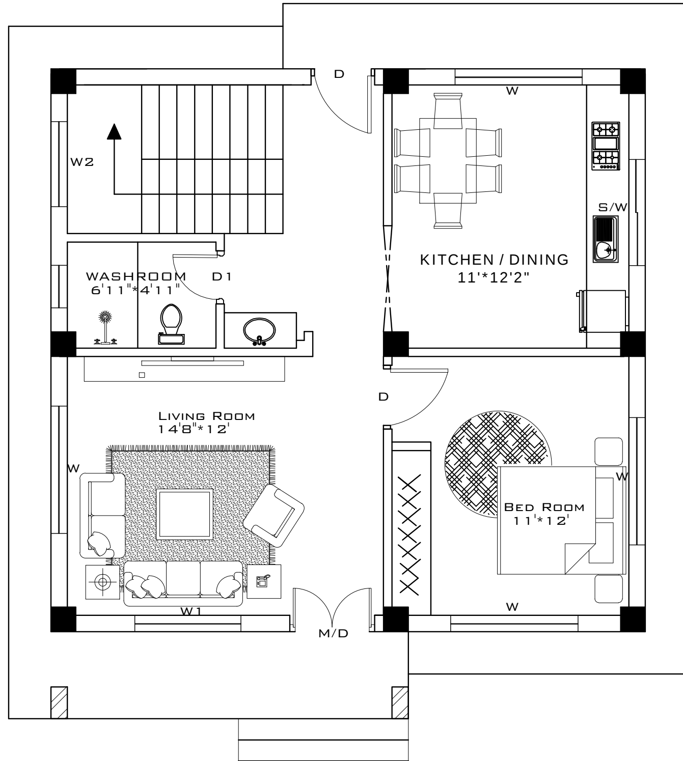
GROUND FLOOR PLAN AREA: 66.86 SQ.M.(719.41 SQ.F.)
